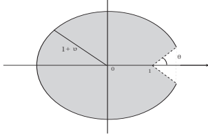
Figure 1: \Delta_1(\nu, \theta) .
