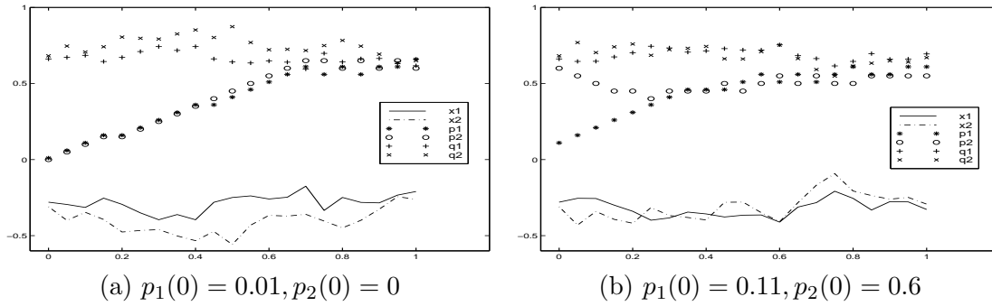
FIGURE 3.2. The trajectories for the attenuation x_i and power p_i ; The power weight \lambda = 0.001
