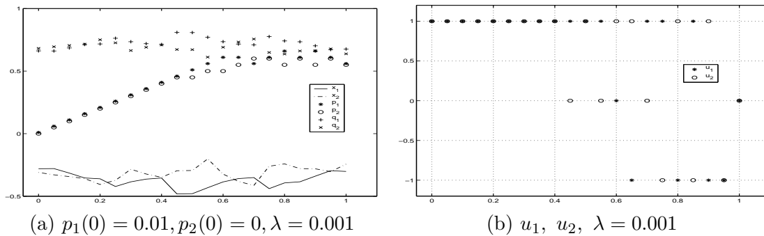
FIGURE 3.4. Left: the trajectories for the attenuation x_i and power p_i ; Right: the control input u_i of two users; The power weight \lambda = 0.001
