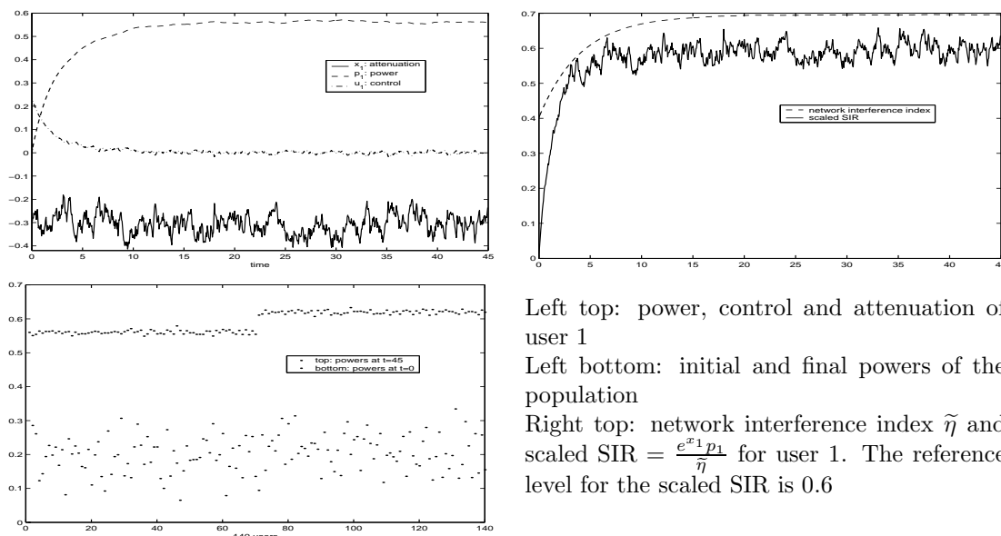
FIGURE 5.6. The power adjustment of user 1 and the behaviour of the population with the single user based control law
