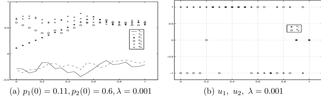
FIGURE 3.5. Left: the trajectories for the attenuation x_i and power p_i ; Right: the control input u_i of two users; The power weight \lambda = 0.001
